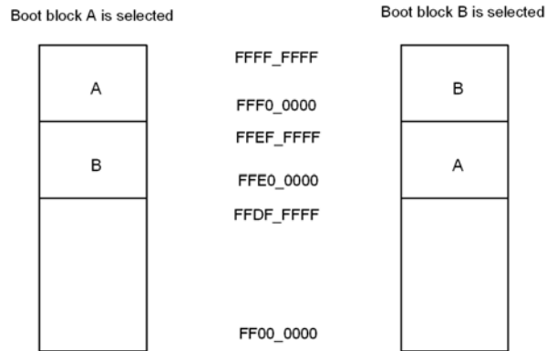
Figure 1-1 Boot Flash Bank
