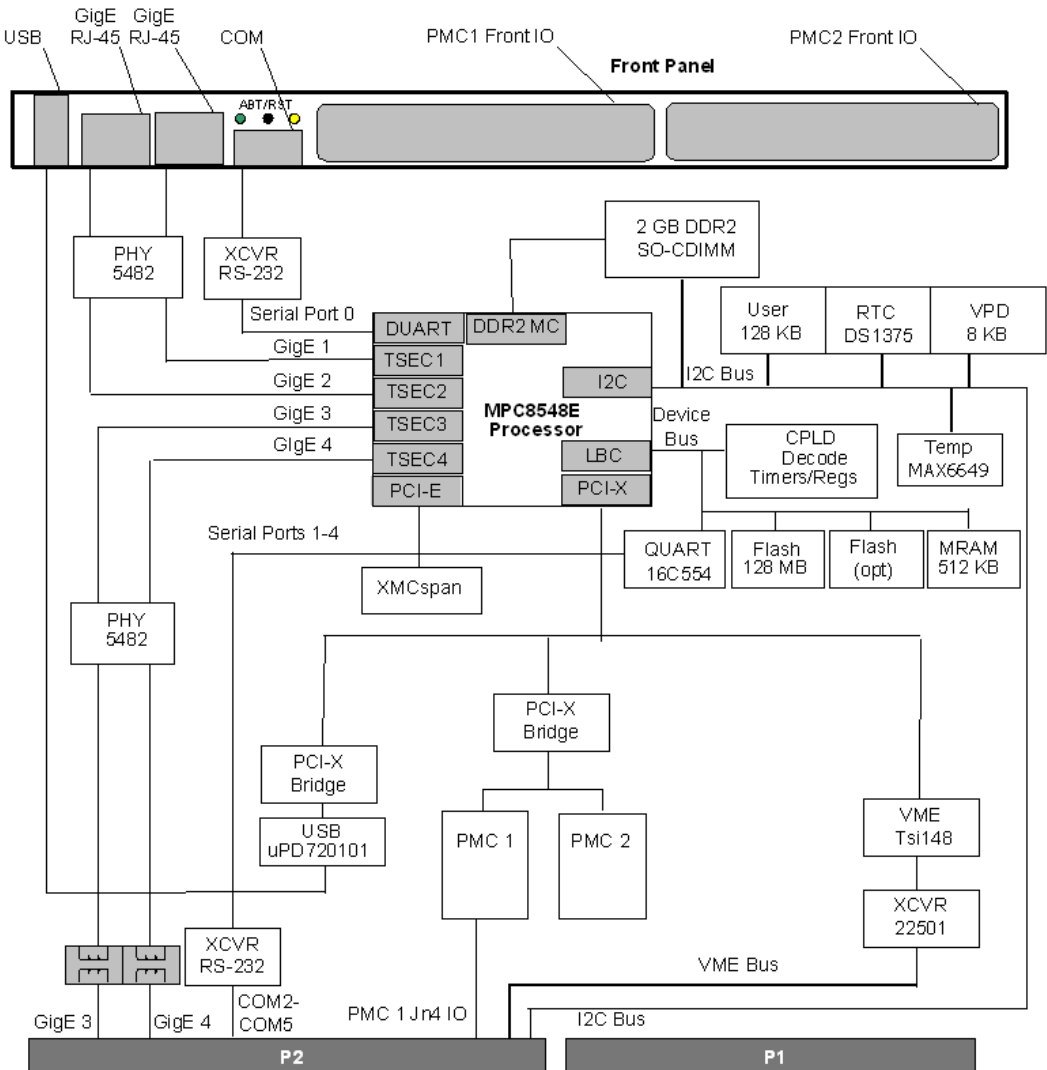
Figure 1-1 Block Diagram
