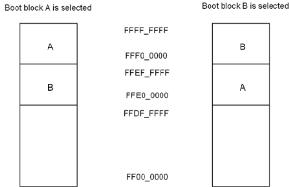
Figure 3-1 Boot Flash Bank
