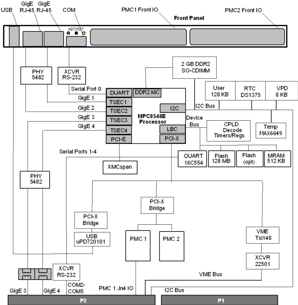
Figure 1-1 Block Diagram
