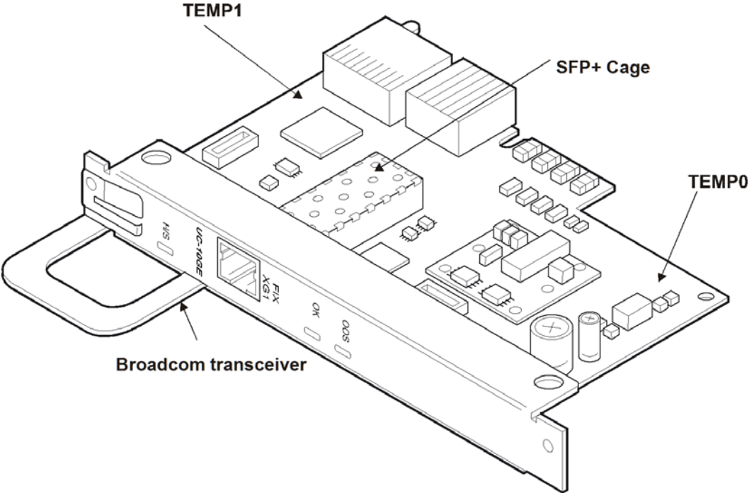
Figure 3-1 Temperature Sensors on Front Centellis 2x00 User Card-10GE
